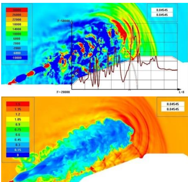
Fig. 7. Pressure distribution and density in plane of main ERS nozzle at Mach = 0
