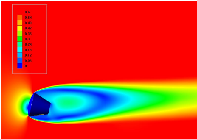
Fig 3. Mach number distribution over spacecraft before lid separation
