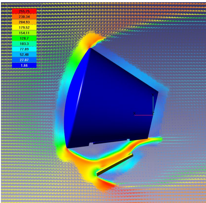
Fig. 4. Velocity distribution after lid separation
