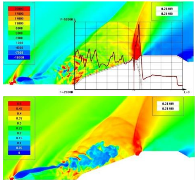
Fig. 8. Pressure distribution and density in plane of main ERS nozzle at Mach=1.5
